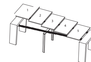
O/400.L 5 allunghe (extensions) aperto max (max extension): cm 270(45+5x45)x90x75h chiuso (closed): cm 90x45x75h
